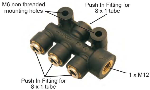
5 Port Plastic Manifold Valve Part No. 7992P
