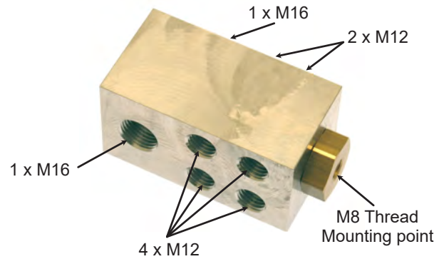
8 Port Aluminium Manifold Valve c/w Plug Part No. 7994
