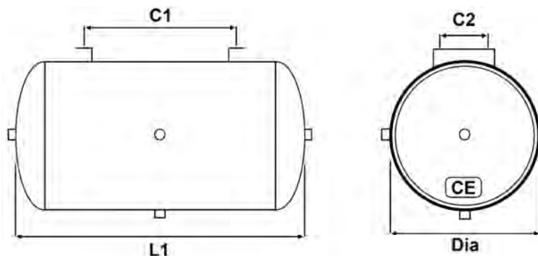
Steel Side Mounted 4 Port Reservoirs
