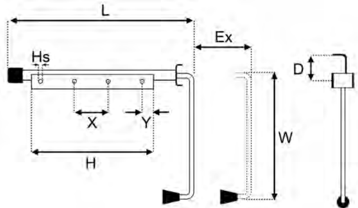
Spring Loaded Door Retainer
