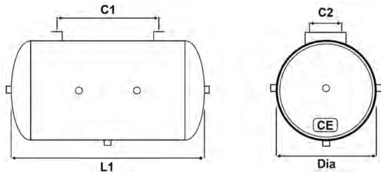
Steel Side Mounted 6 Port Reservoirs
